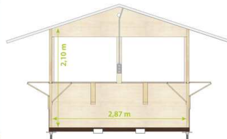
VISTA INTERNO LATO FRONTALE VORDERANSICHT INNEN INTERIOR VIEW FRONT SIDE
