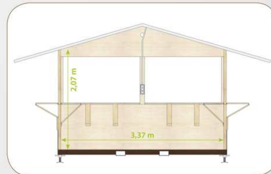
VISTA INTERNO LATO FRONTALE VORDERANSICHT INNEN INTERIOR VIEW FRONT SIDE
