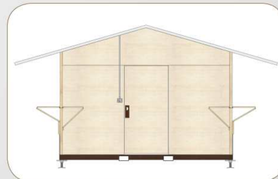
VISTA INTERNO LATO POSTERIORE RÜCKANSICHT INNEN INTERIOR VIEW BACK SIDE
